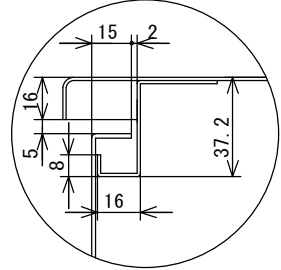
A部断面詳細 (1/2)
