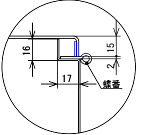
B部断面詳細 (1/2)
