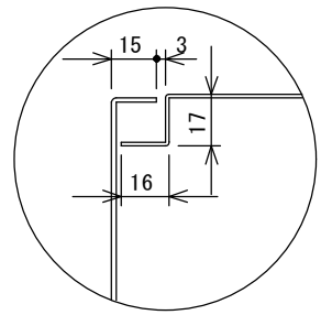
A部断面詳細 (1/2)
